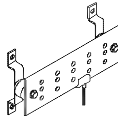
Ground Bar with wall mounting brackets, insulators, and a 25' ground conductor
